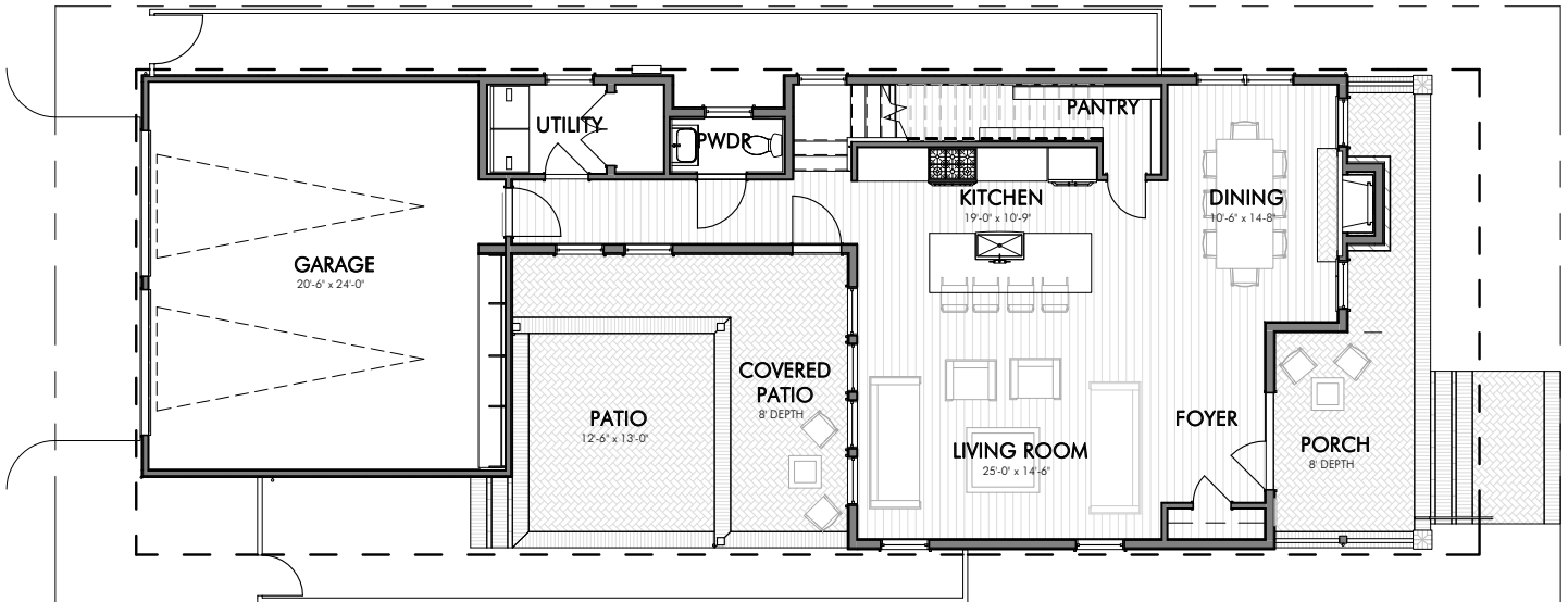
FIRST FLOOR
