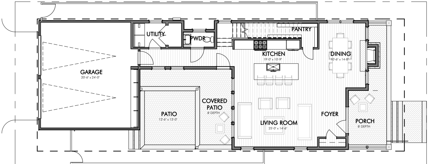
FIRST FLOOR
