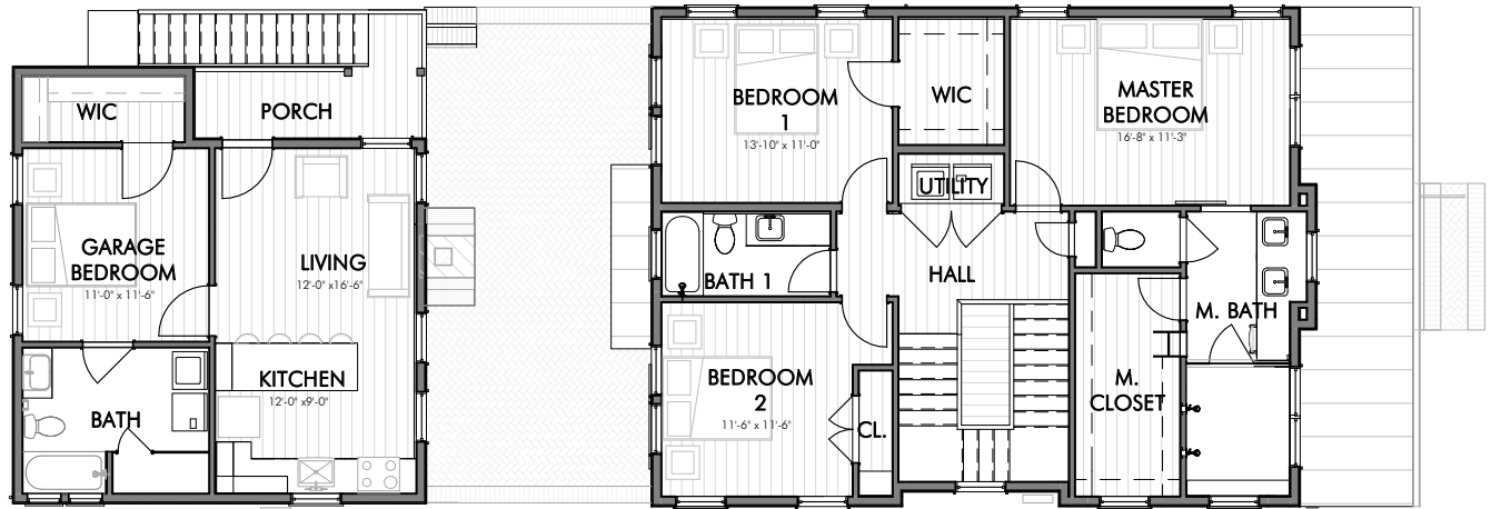
SECOND FLOOR
