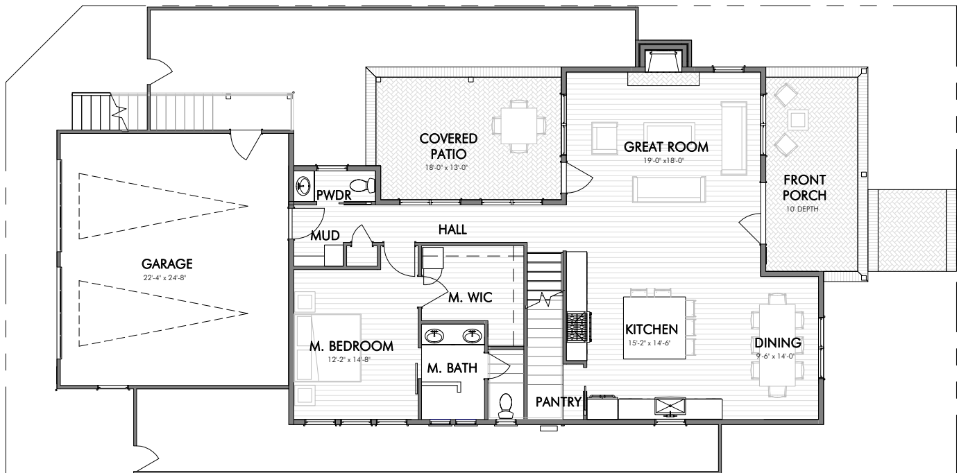
FIRST FLOOR
