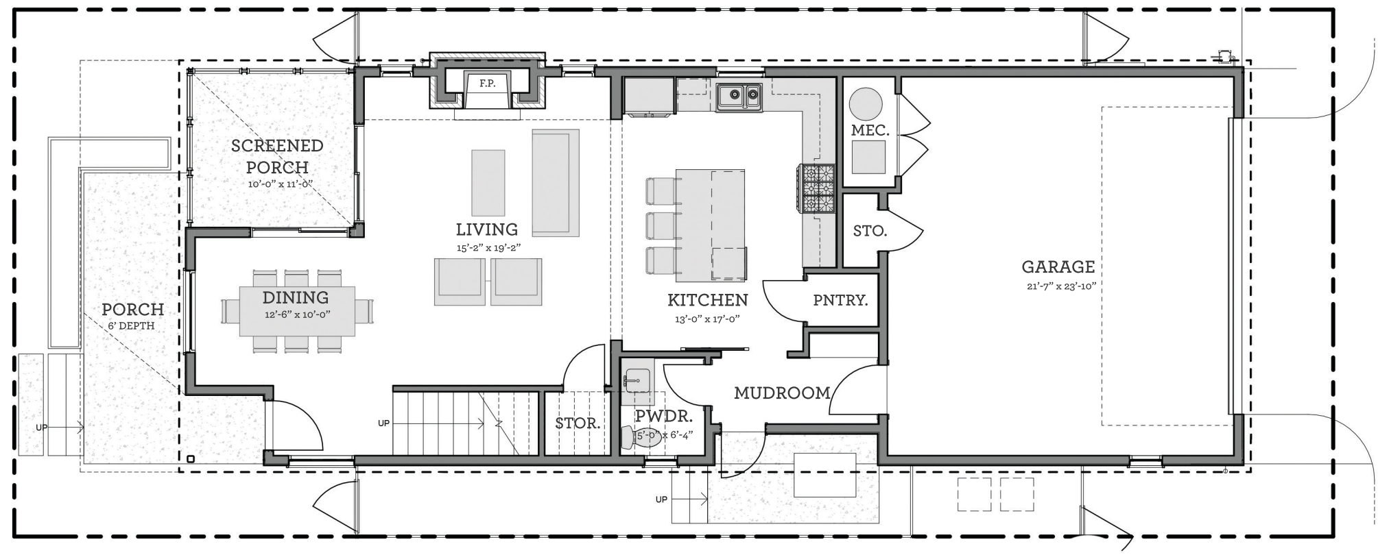
⊕ FIRST FLOOR SCALE 1/8" = 1'-0"
