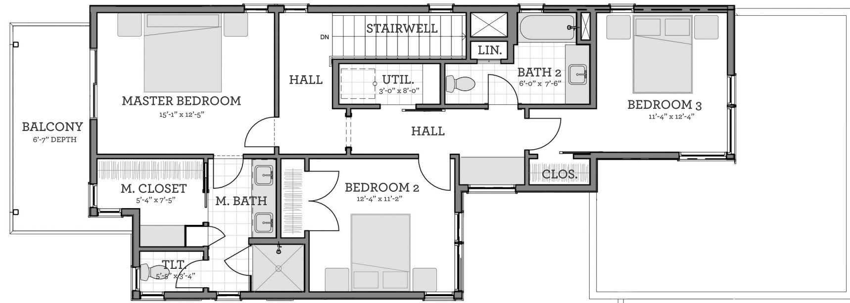
⊕ SECOND FLOOR SCALE 1/8" = 1'-0"
