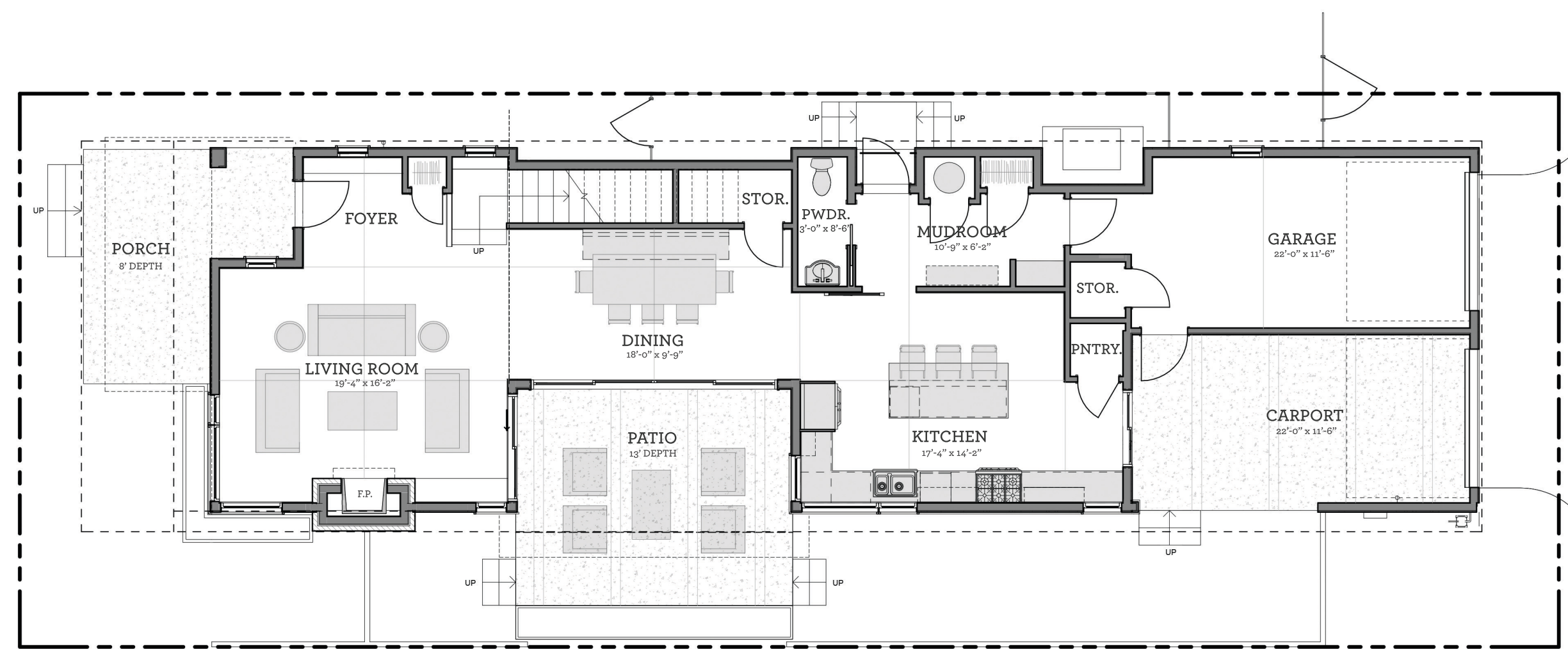
⊕ FIRST FLOOR SCALE 1/8" = 1'-0"
