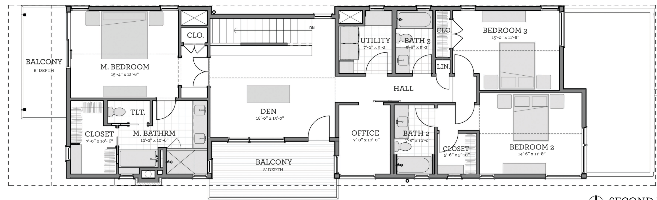
⊕ SECOND FLOOR SCALE 1/8" = 1'-0"
